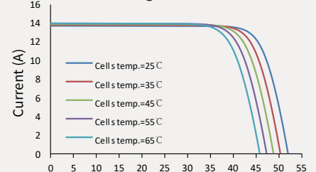
Current-Voltage (580W)
